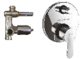
Push type single lever concealed diverter system consisting of Exposed part (lever, turn type knob, flange) and Concealed part (35 mm cartridge with button assembly, cartridge sleeve) Exposed part F1015701 Concealed part F4010108
