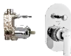
5-way (3 inlets + 2 outlets) single lever concealed diverter system consisting of Exposed part (lever, tip ton knob, flange) and Concealed part (cartridge with button assembly, cartridge sleeve)
