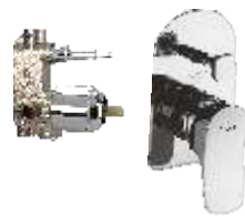
5-way (3 inlets + 2 outlets) single lever concealed diverter system consisting of Exposed part (lever, tip ton knob, flange) and Concealed part (cartridge with button assembly, cartridge sleeve)
