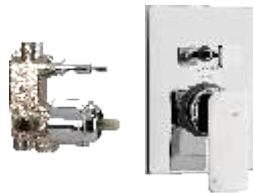
5-way (3 inlets + 2 outlets) single lever concealed diverter system consisting of Exposed part (lever, tip ton knob, flange) and Concealed part (cartridge with button assembly, cartridge sleeve) Exposed part F1005711 Concealed part F4020101
