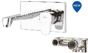
Wall mounted single lever basin mixer consisting of exposed part and concealed part Exposed part F1020473 Concealed part F4065101
