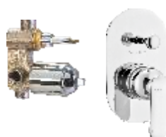
High flow single lever concealed diverter system consisting of Exposed part (lever, tip ton knob, flange) and Concealed part (45 mm cartridge with button assembly, cartridge sleeve)
