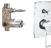
Single lever concealed diverter system consisting of Exposed part (lever, tip ton knob, flange) and Concealed part (35 mm cartridge with button assembly, cartridge sleeve) Exposed part F1099701 Concealed Part F4010103
