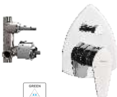
Turn type single lever concealed diverter system consisting of exposed part (lever, turn type knob and 2mm thick sheet metal wall flange) and concealed part (35 mm cartridge with button assembly, cartridge sleeve) Exposed part F1013702 Concealed part F4010107
