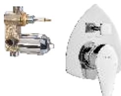
High flow single lever concealed diverter system consisting of Exposed part (lever, tip ton knob, flange) and Concealed part (45 mm cartridge with button assembly, cartridge sleeve) Exposed part F1013721 Concealed Part F4030101
