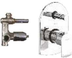
Push type single lever concealed diverter system consisting of Exposed part (lever, tip ton knob, wall flange) and Concealed part (35 mm cartridge with button assembly, cartridge sleeve) Exposed part F1019701 Concealed Part F4010108
